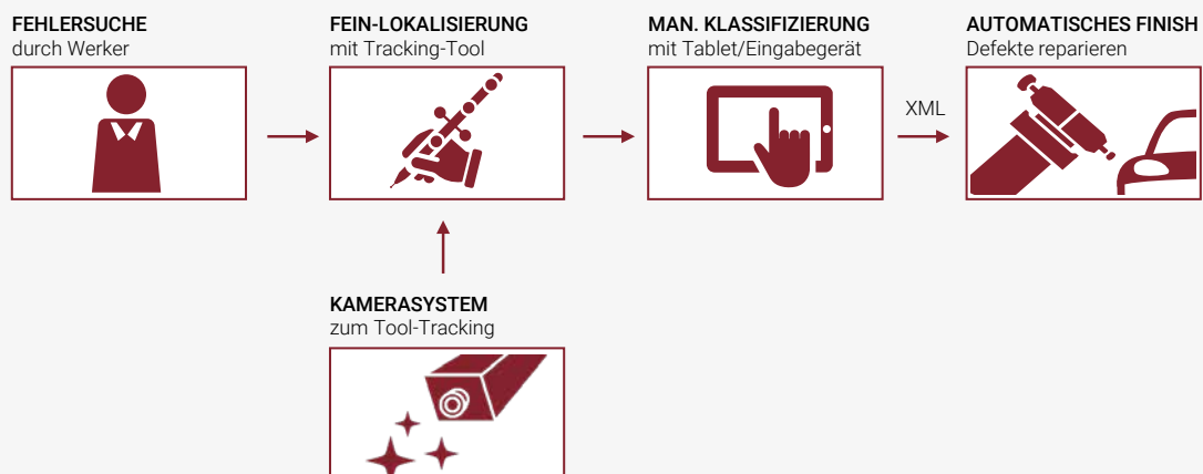
Abb. 15: Schema MDD Basic
