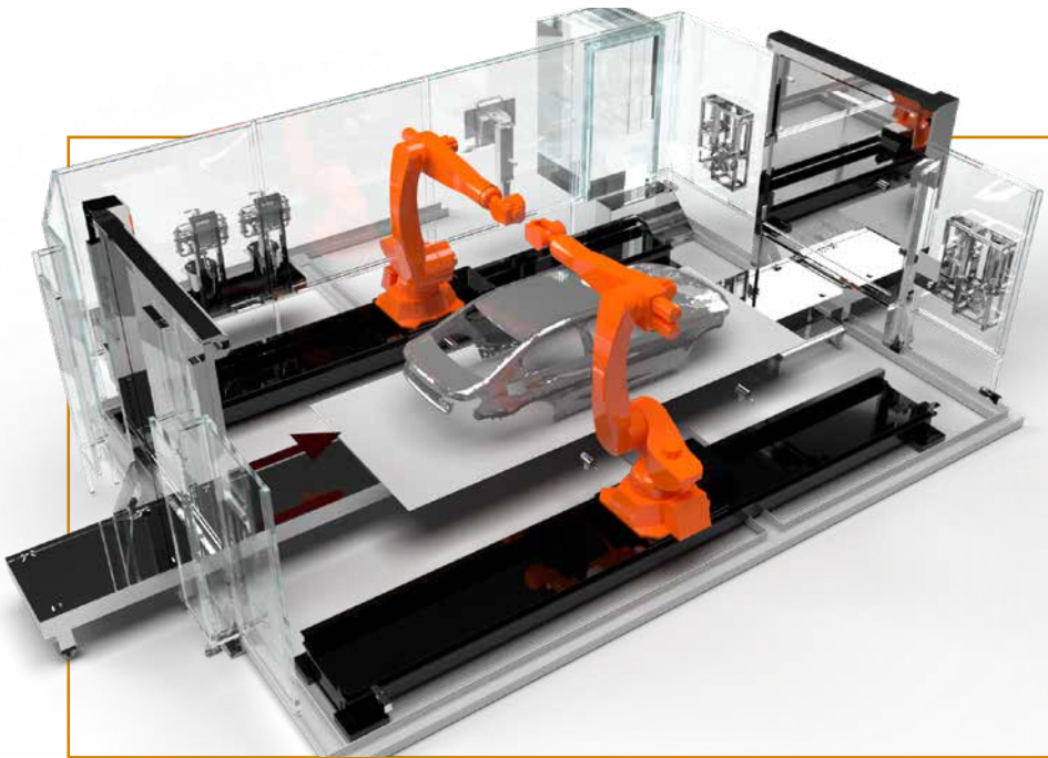
Automatic surface treatment after top coat and clear coat application
