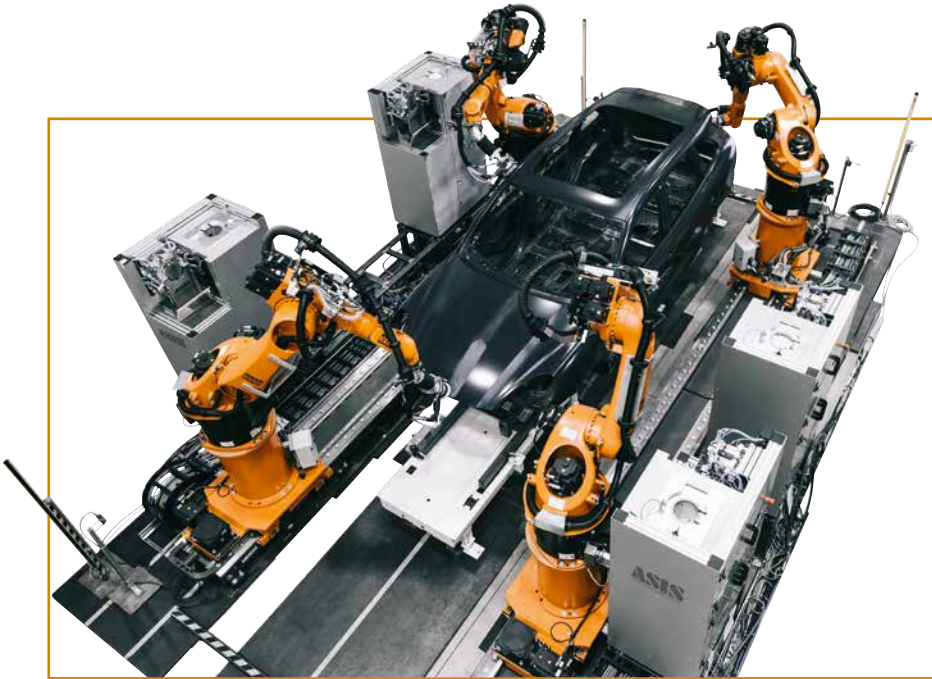
Fully automated sanding system for primer.
