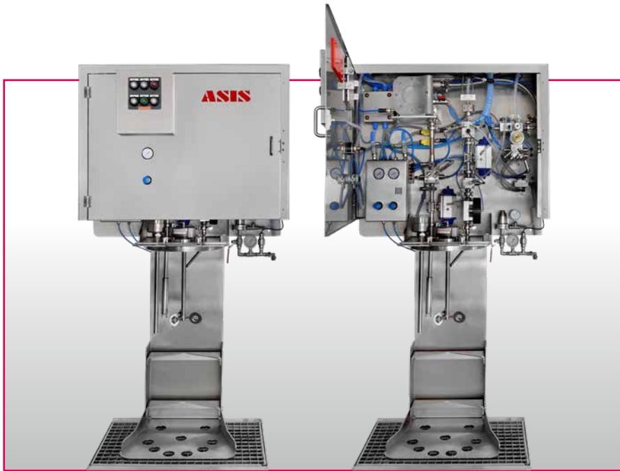
The ASIS Special Color Supply System®: fast color change with low paint loss for low operating costs.
